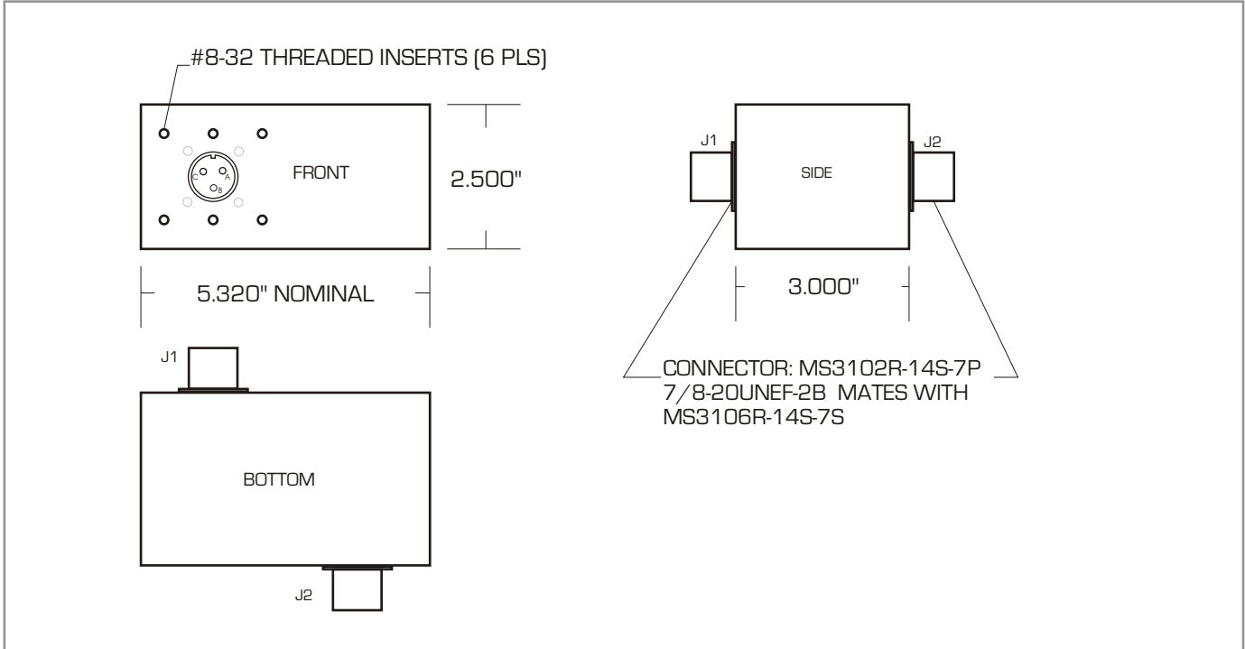
OUTLINE DRAWING
